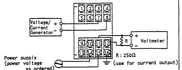
Fig.12 Wiring of Calibration Equipment
