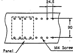
Fig.9 Terminal Arrangement
