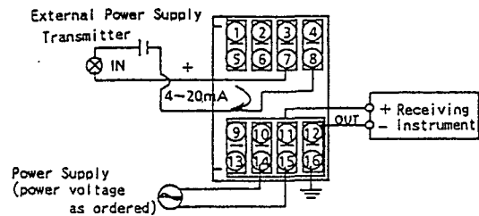
Fig.12 Wiring of Calibration Equipment
