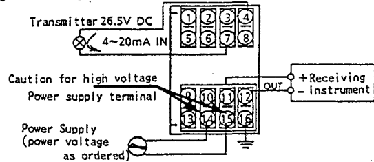
Fig.11 Wiring Diagram (2)
